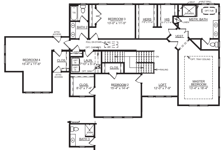
OPTIONAL BATH 3 AT BEDROOM 2
